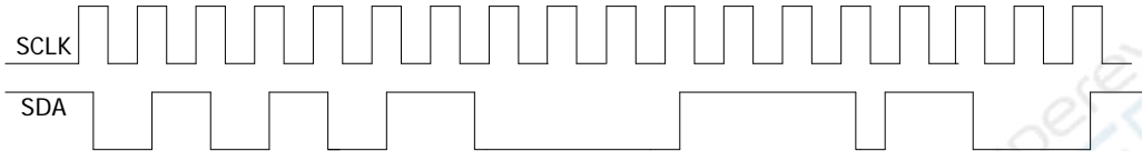
Figure 8-5 I2C Serial Bus
