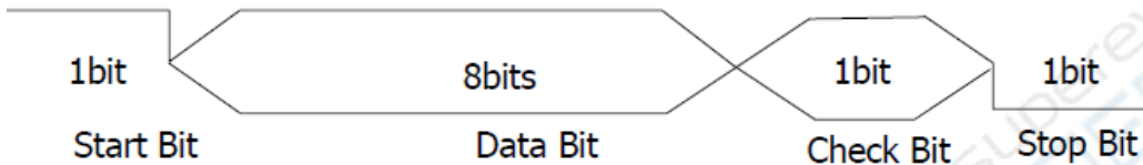
Figure 5-13 RS232 Trigger
