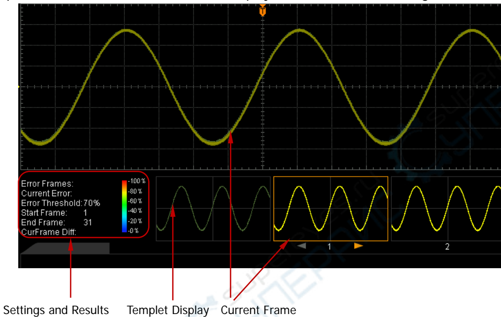
Figure 11-3 Waveform Analysis
