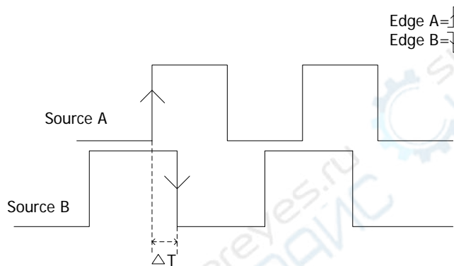
Figure 5-9 Delay Trigger
