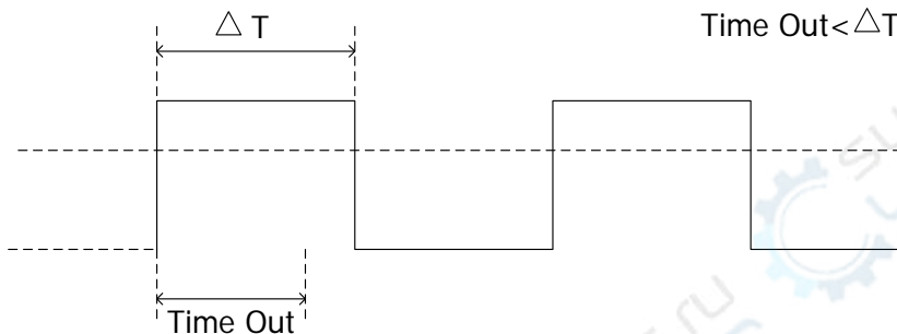
Figure 5-10 TimeOut Trigger
