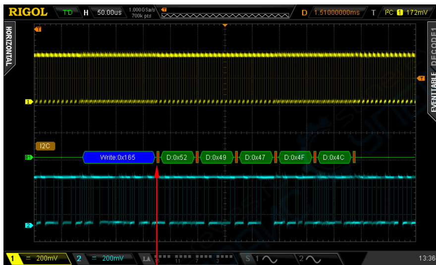
Figure 8-9 Error Expressions during Decoding
